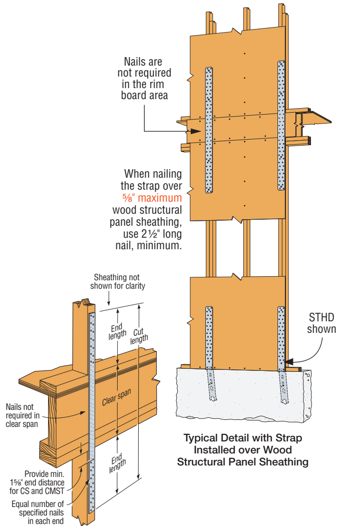
Floor-to-Floor Tie Installation Showing a Clear Span
