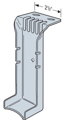
HF26N (HF36N similar) Dimples hold joist securely in place.
