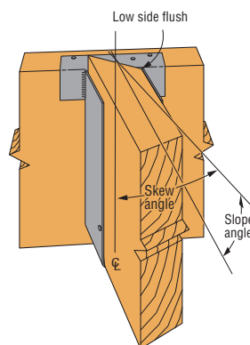
Typical WP sloped down, skewed right with type A hanger (joist end must be bevel cut). When ordering, specify low side flush, center flush or high side flush.
