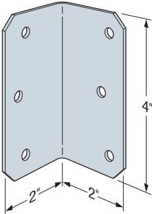
ML24Z (ML26Z similar)
