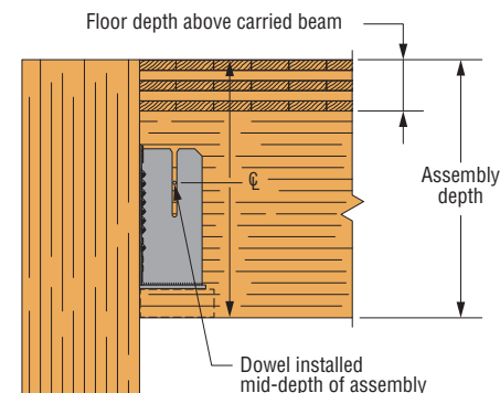
Beam-to-Column Assembly with CLT Floor Above (fasteners not shown for clarity)
