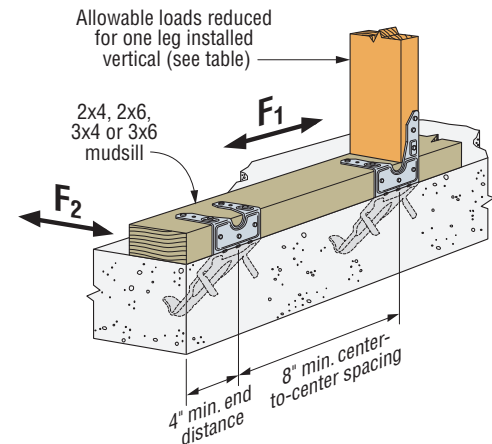
Typical MASA/MASAP Installation on Sill Plate
