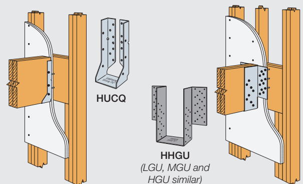
HUCQ Installed Over Two Layers of 5/8\"/&gt;
