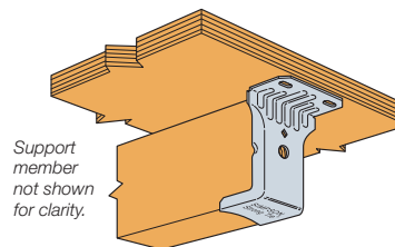
Typical HF24N Installation (HF34N similar)
