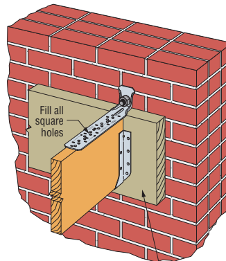
Typical LTTP2 Installation for Solid Sawn Joist
