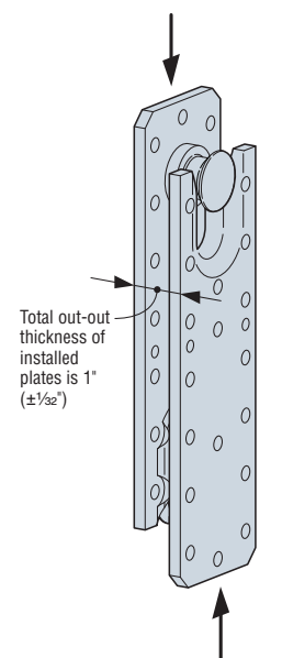
Assembly Thickness and Fit-Up Tolerance
