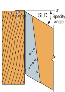
Typical Sloped Down Installation with Full Backing
