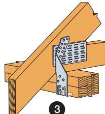
TSP Installation
