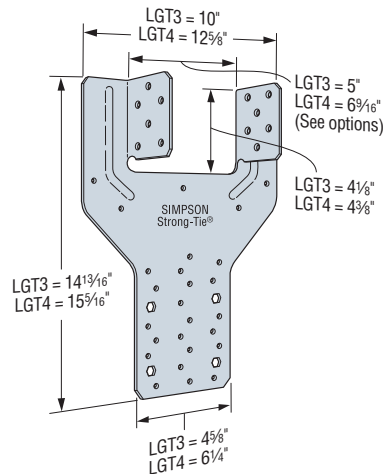
LGT3-SDS2.5 (LGT4-SDS3 similar)
