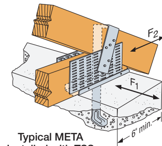
Typical HETA20 Installation (all others similar)
