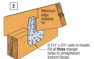
H14 Installation to Double 2x Header
