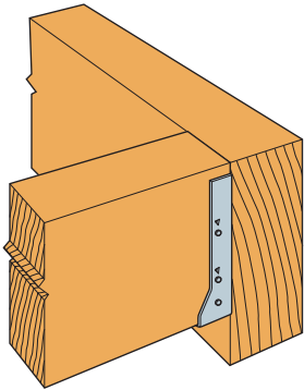
Typical HUC Installed on a Beam
