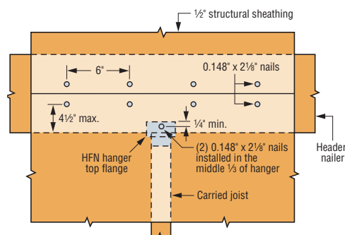
HFN Panelized Installation (plan view)
