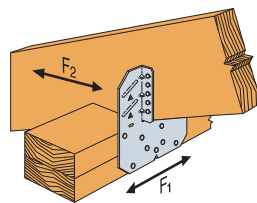
H10A Installation
