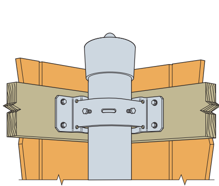
Typical PGTIC2Z-R Fence Installation
