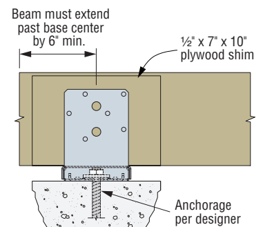
Figure 4 — ABU with Beam Installation
