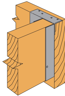
Typical WP Top Flange Offset Left
