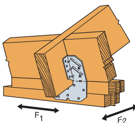
H10A Field-Bent Installation
