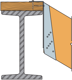
Typical Sloped Down on Nailer Non-Backed
