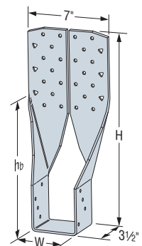
THGQ3.62-SDS (others similar)
