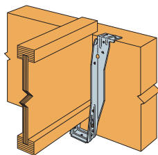
Step 2 Slide the I-joist downward into the ITS until it rests above the Strong-Grip™ seat.
