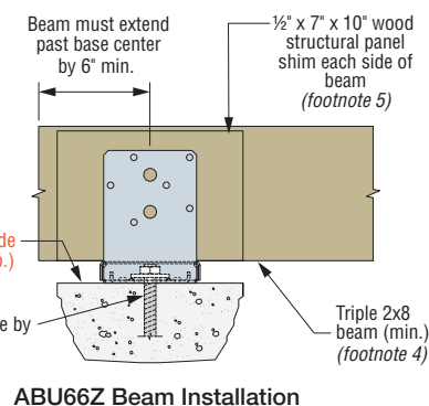
ABU66Z Beam Installation
