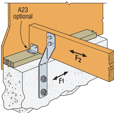
Typical FJA Installation Foundation to Joist
