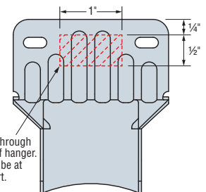
HF26N (HF36N similar) Dimples hold joist securely in place.
