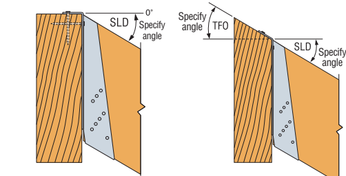
Typical Sloped Down Installation with Full Backing
