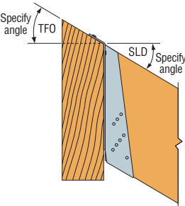
Typical Sloped Down with Top Flange Open
