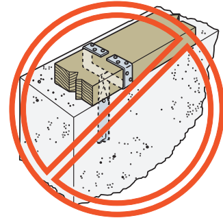
MAB Misinstallation (MAB straps must be separated before the concrete is poured or installed through ¾"-diameter hole)
