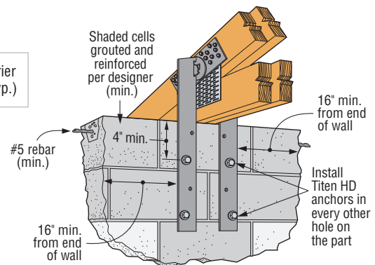
Typical FGTR Double Installation
