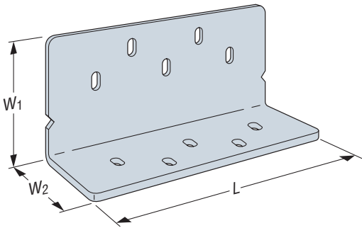
HSLQ37 (HSLQ312, HSLQ47, HSLQ412 similar)
