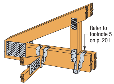
Typical THA29 Top Flange Installation
