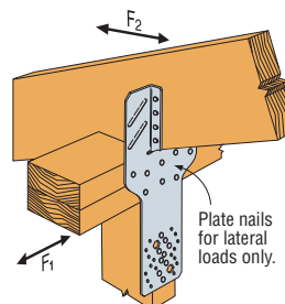
H10S Installation
