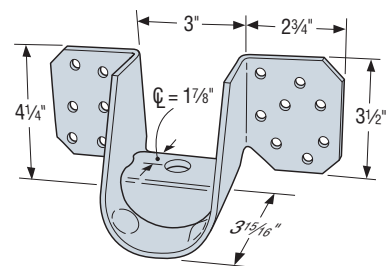
VGT US Patent 7,707,785
