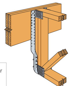
THA422 Face-Mount (Min.) Installation
