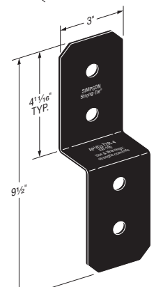
APVDJT2R-4 (others similar)
