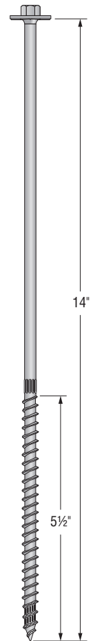
Strong-Drive SDWH Timber-Hex HDG Screw (included)
