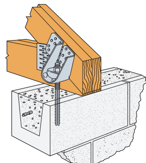
Typical VGTR Installation (VGTL similar)
