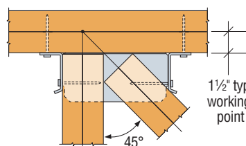
THJU26-W Top View Two-Ply Hip / Two-Ply Jack Installation
