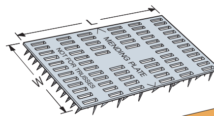
MP36 (other sizes similar)
