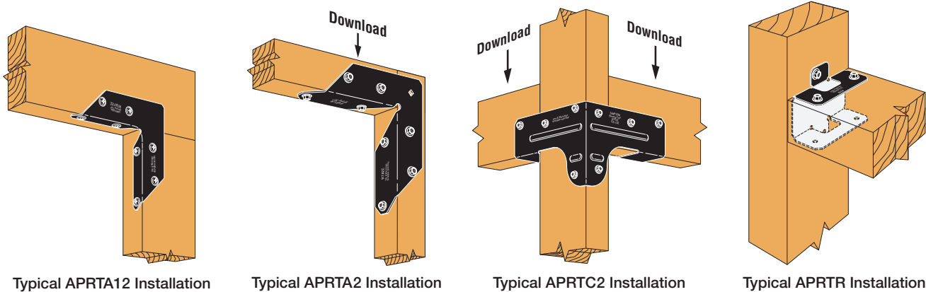
Typical APRTA12 Installation
