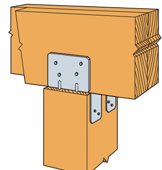
Typical LPC4Z Installation
