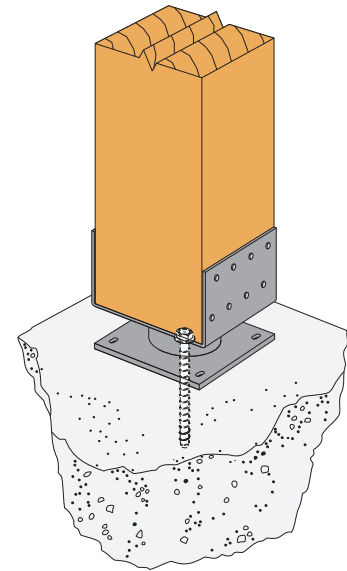
Typical ECB Concrete Installation
